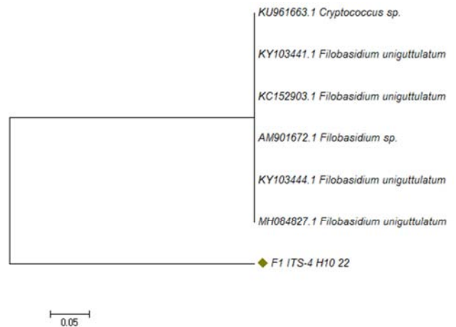
Figure 5. Phylogenetic tree showing species relatedness of isolate F1.
