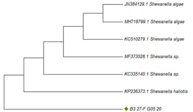
Figure 4. Phylogenetic tree showing species relatedness of isolate B3.
