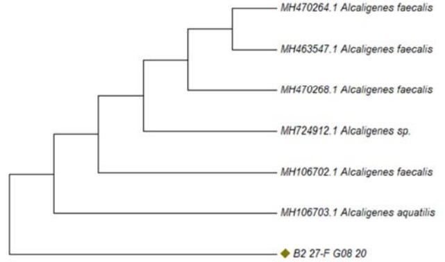
Figure 3. Phylogenetic tree showing species relatedness of isolate B2.
